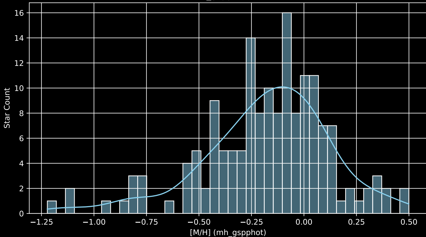
APOGEE DR17 Field: [235+12 [M/H] (mh_gspphot) (n= 160)
