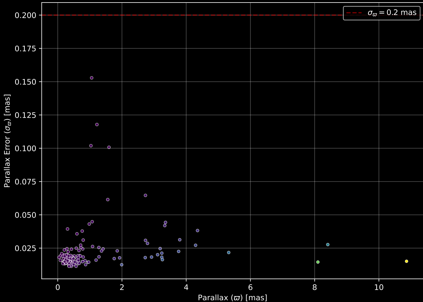
APOGEE DR17 Field: [235+12] Parallax Quality (n= 161)
