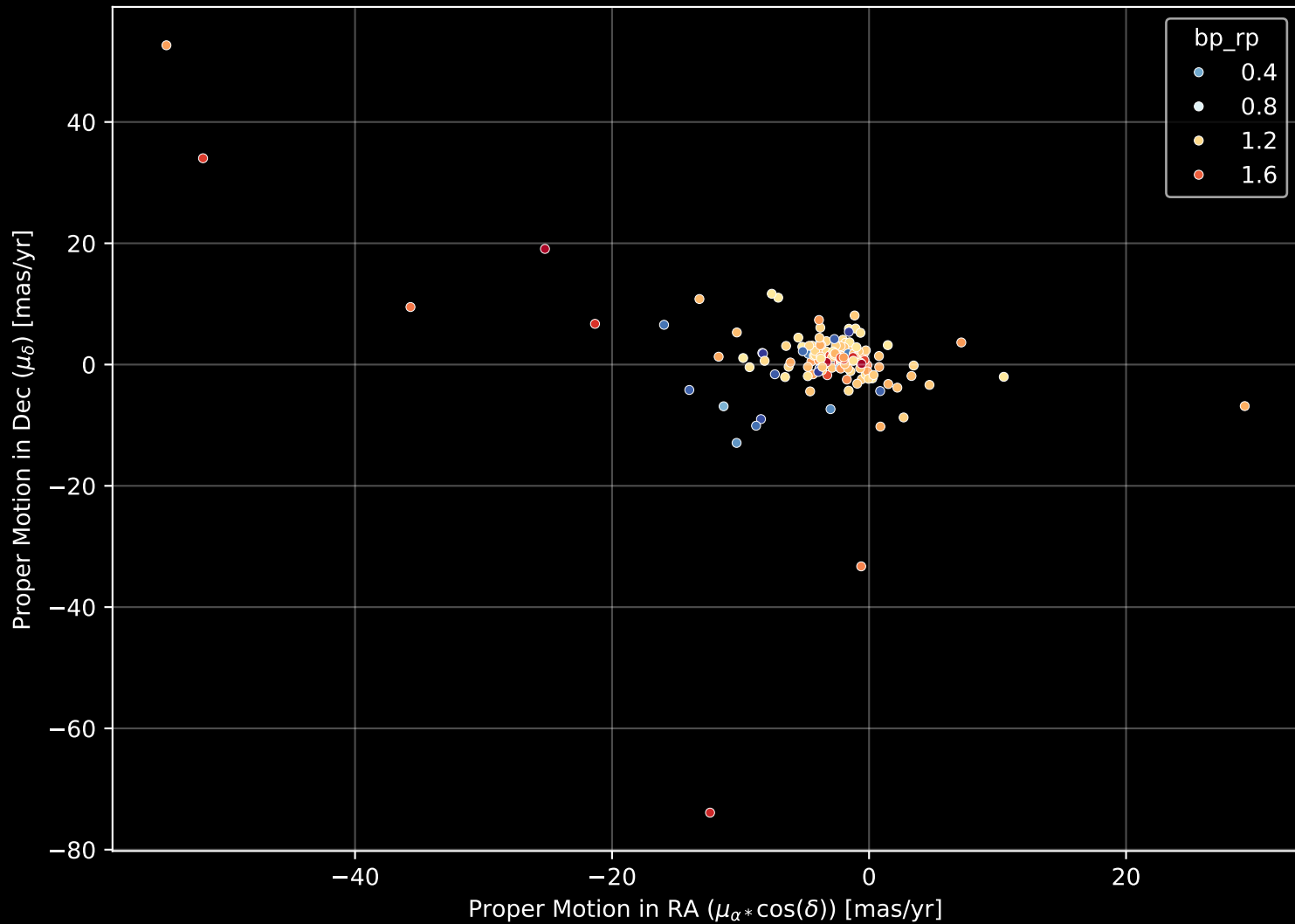
APOGEE DR17 Field: [235+12] Proper Motion Diagram (n= 161)
