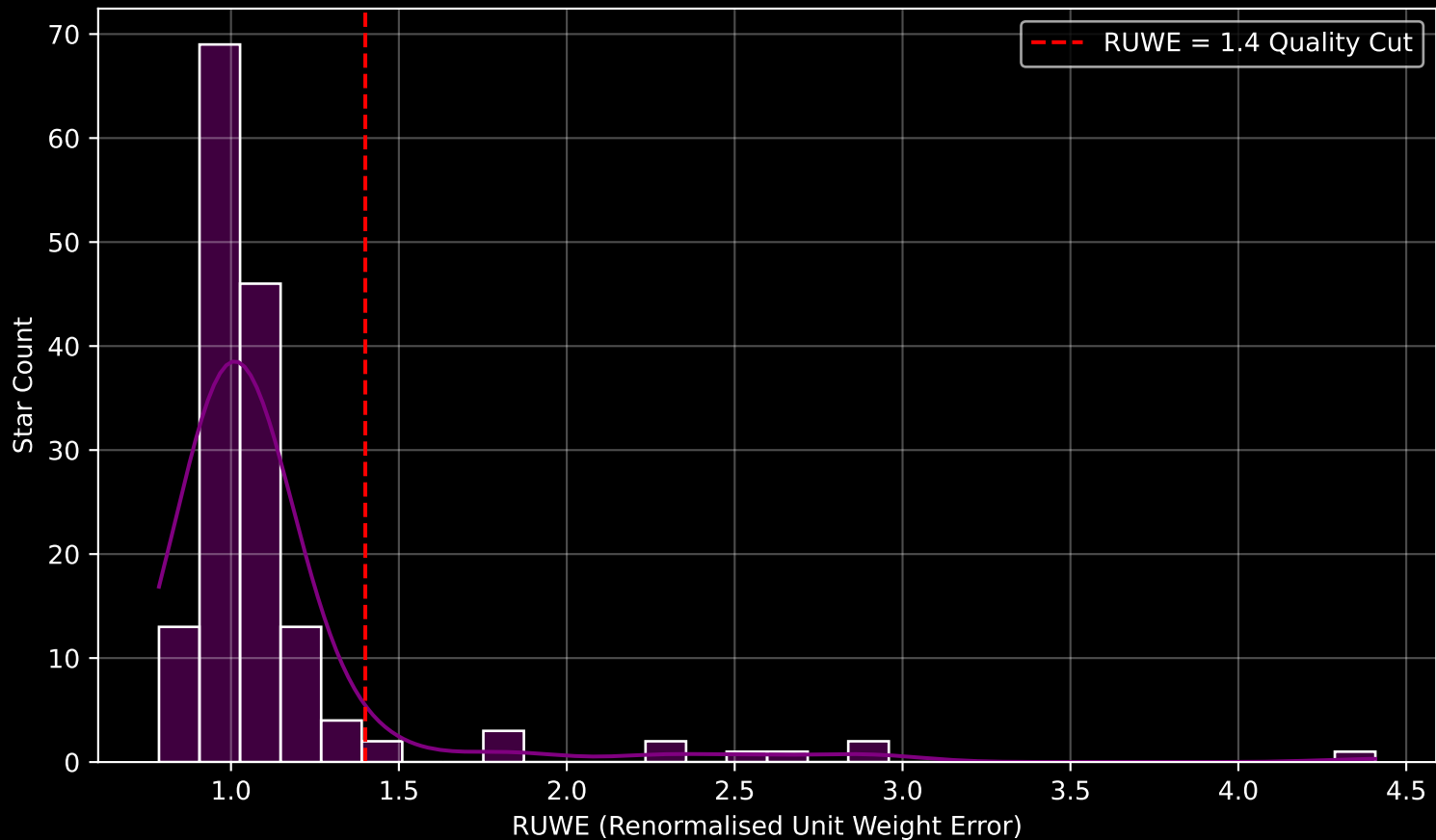
GAPOGEE DR17 Field [235+12] RUWE Distribution (n= 157)
